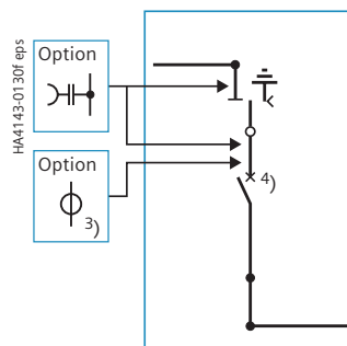
Type L1(r, T), 630 A 750 mm wide
