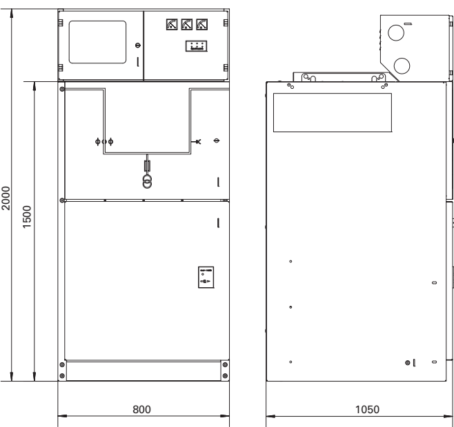
Type M panel dimension for 24kV
